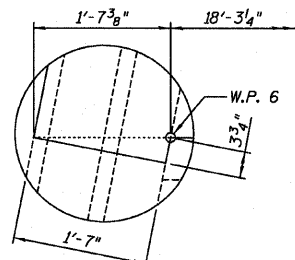
DETAIL F
