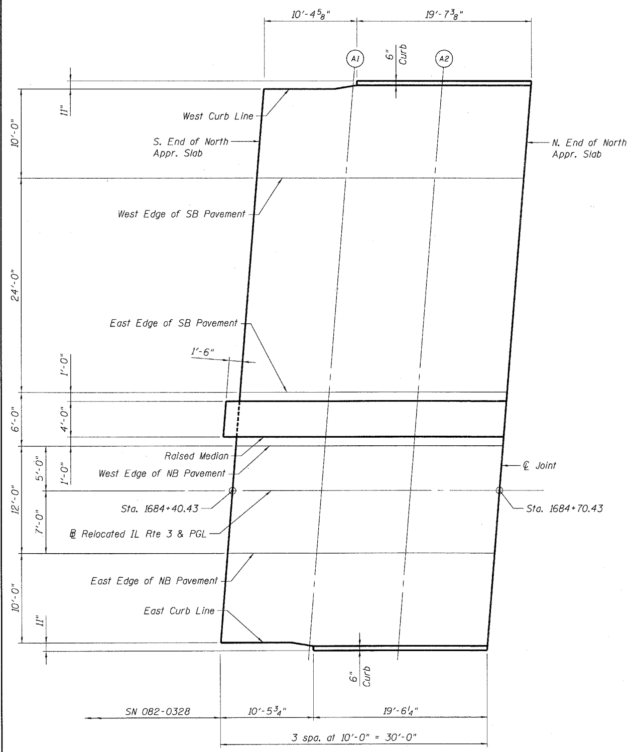
PLAN North Approach SN 082-0328
