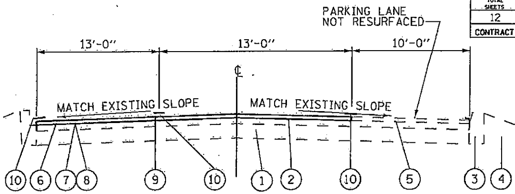
PROPOSED TYPICAL SECTION STA. 105±68 TO STA. 140±73 (LOOKING EAST)
