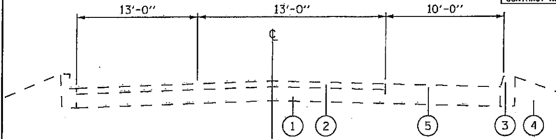
EXISTING TYPICAL SECTION STA. 105±68 TO STA. 140±73 (LOOKING EAST)
