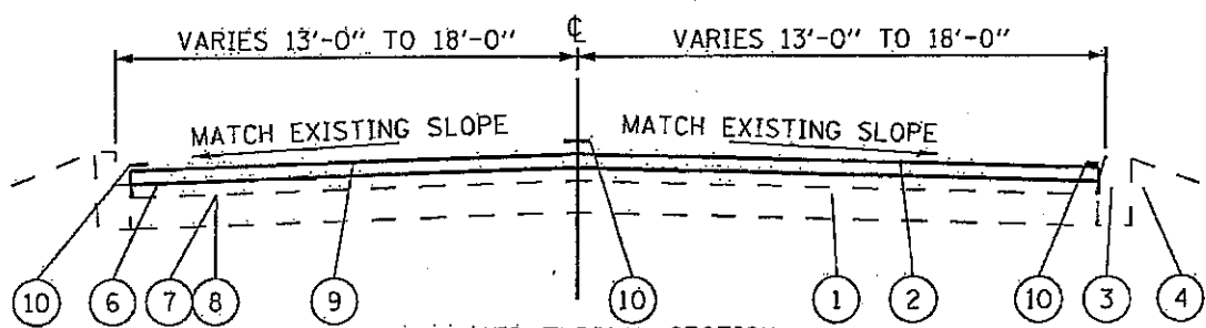
PROPOSED TYPICAL SECTION STA. 150±91 TO STA. 152±72 STA. 188±45 TO STA. 188±95
