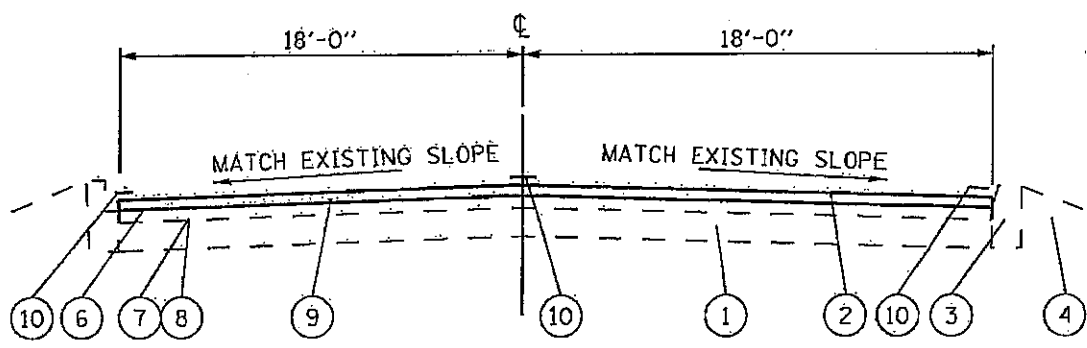
PROPOSED TYPICAL SECTION STA. 140±73 TO STA. 150±91 STA. 170±01 TO STA. 188±45
