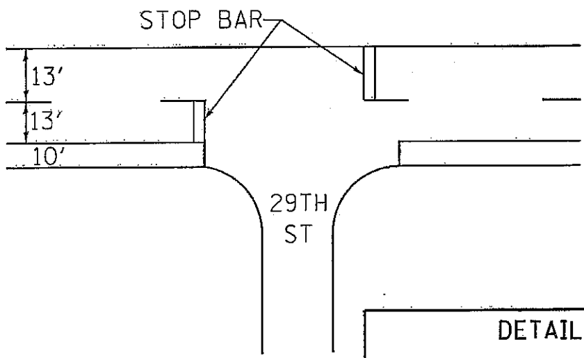
SIDEROAD DETAIL
