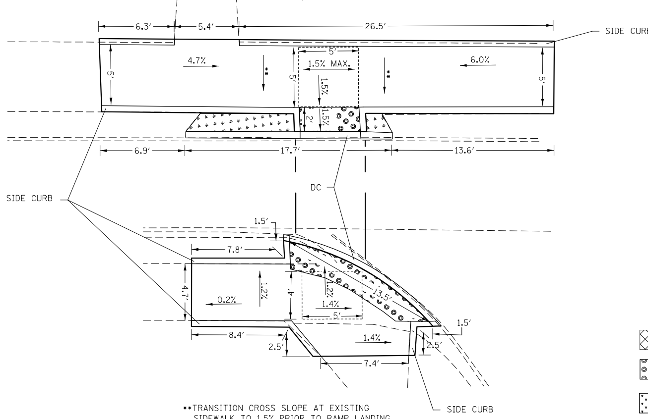
PROPOSED CROSSWALK AT STA 16+33
