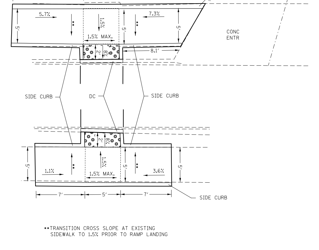
PROPOSED CROSSWALK AT STA 19+81
