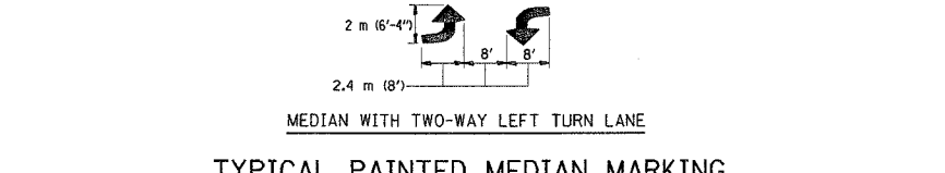
TYPICAL PAINTED MEDIAN MARKING
