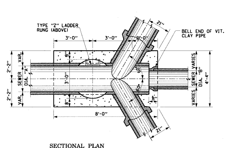
SECTIONAL PLAN
