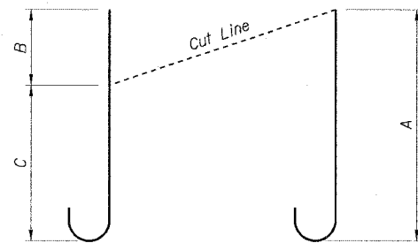
BARS n7(E), n9(E) Cutting Diagram
