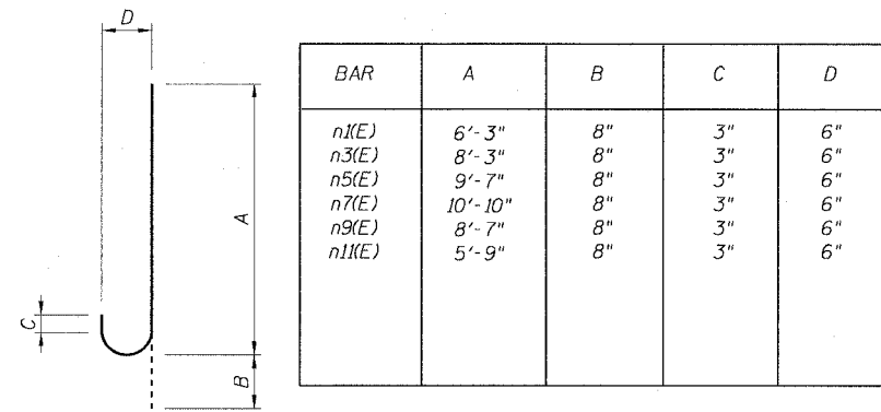
BARS n1(E), n3(E), n5(E), n7(E), n9(E), n11(E)
