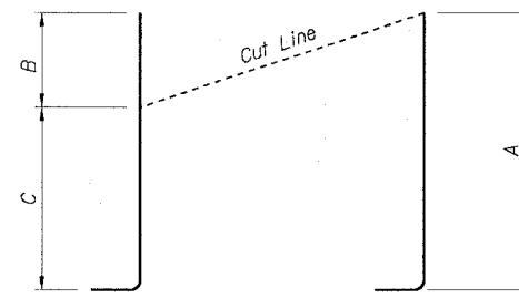
BARS n8(E), n10(E) Cutting Diagram
