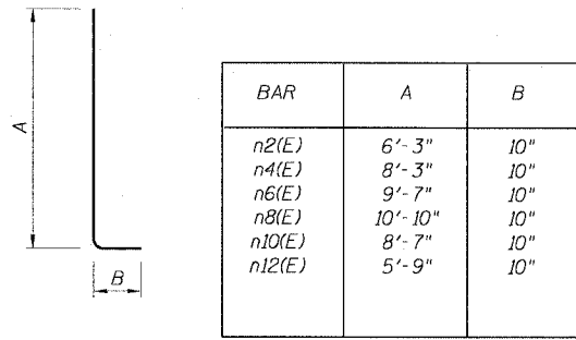
BARS n2(E), n4(E), n6(E), n8(E), n10(E), n12(E)
