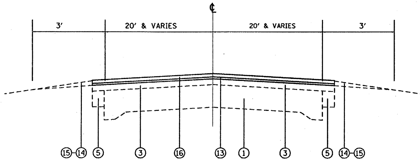
PROPOSED TYPICAL SECTION STA. 29+00± TO STA. 18+90±
