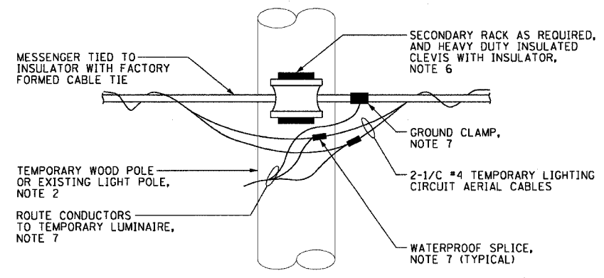
AERIAL CABLE ATTACHMENT DETAIL NOT TO SCALE
