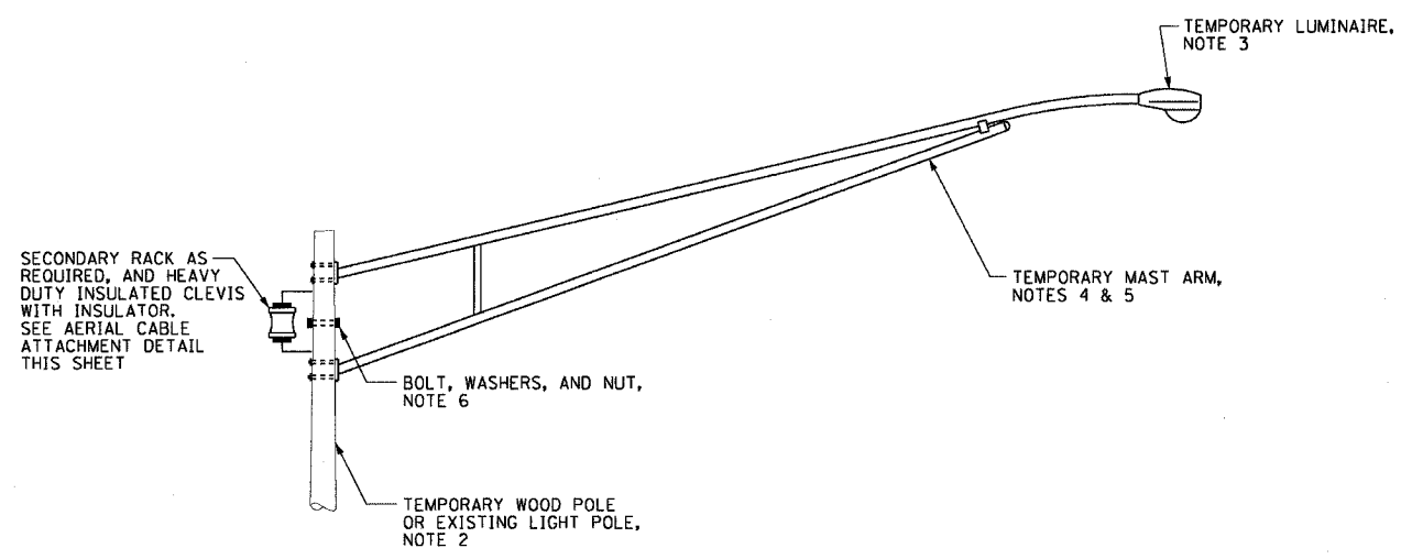
AERIAL CABLE TO TEMPORARY LIGHTING UNIT INSTALLATION DETAIL NOT TO SCALE
