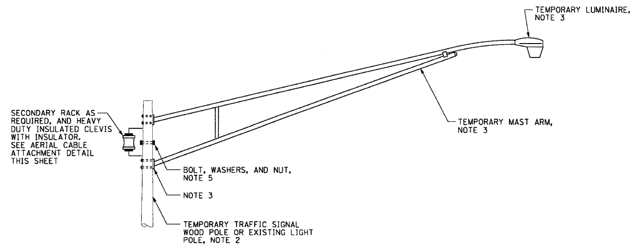
AERIAL CABLE TO TEMPORARY LIGHTING UNIT INSTALLATION DETAIL NOT TO SCALE
