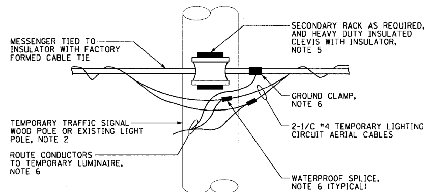
AERIAL CABLE ATTACHMENT DETAIL NOT TO SCALE
