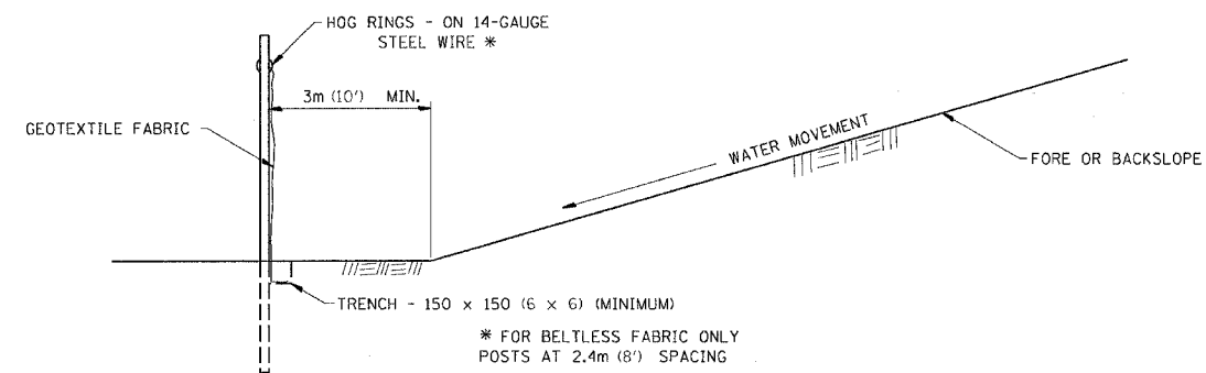
DETAILS OF SILT FENCE
