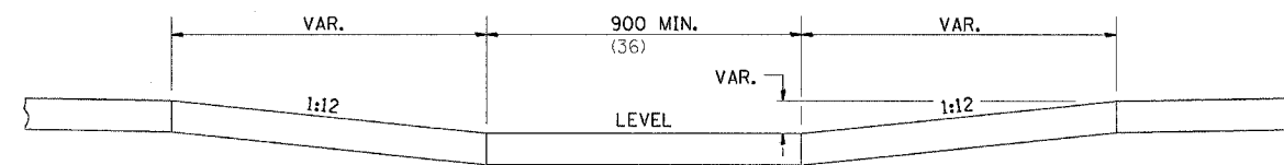
SECTION B-B
