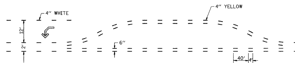
SHORT-TERM PAVEMENT MARKING FOR MEDIANS AND ARROWS
