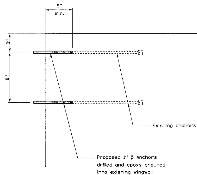
WING WALL ELEVATION
