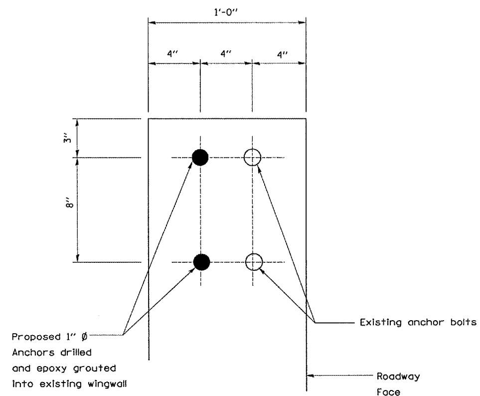
VIEW C-C
