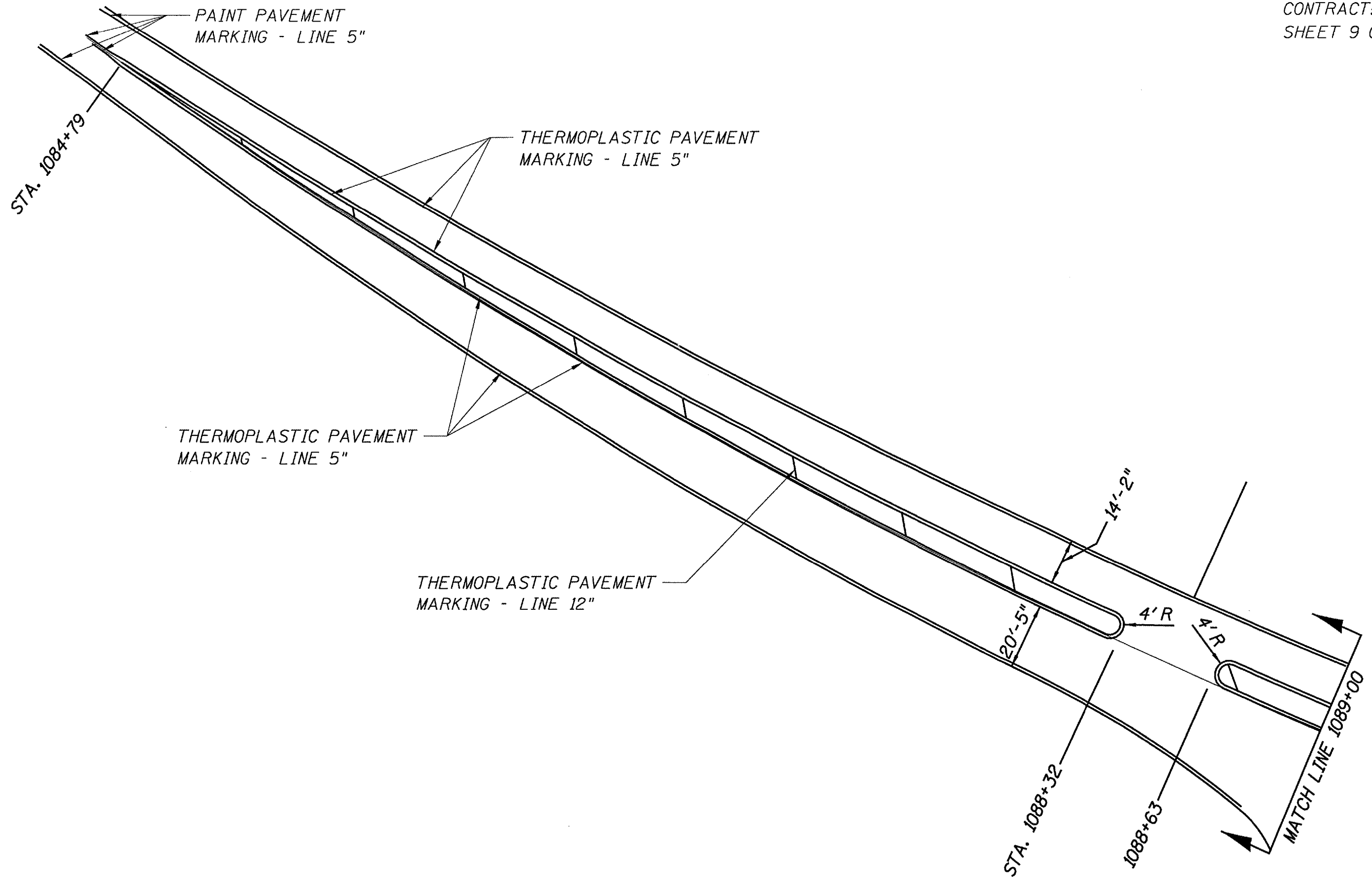
PAVEMENT MARKING DETAILS FAP 757 (OLD US 36) SECTION (21X, 22)RS-7 SCOTT COUNTY
