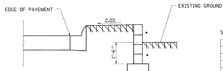
SEGMENTAL CONCRETE BLOCK WALL
