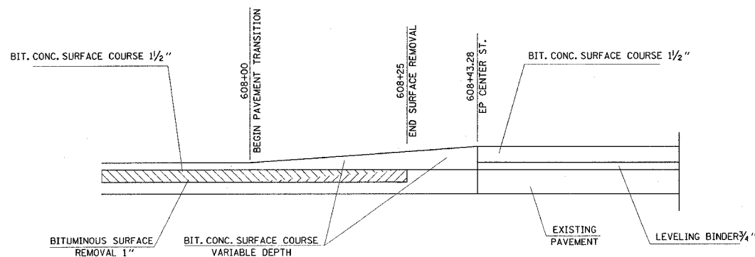
MILLING RESURFACING DETAIL DEWEY ST. AT CENTER ST. (IL 162)
