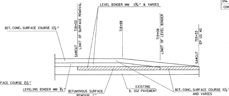
MILLING RESURFACING DETAIL IL 162 AT US 40
