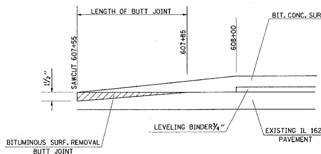
BUTT JOINT DETAIL STA. 608+00
