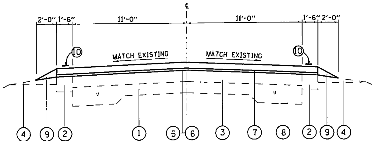
TYPICAL SECTION
