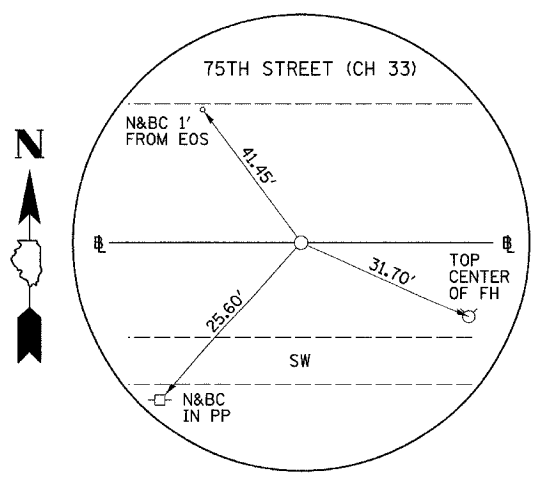
PI STA. 537+36.87 75TH STREET (CH 33) (5/8" I-ROD)
