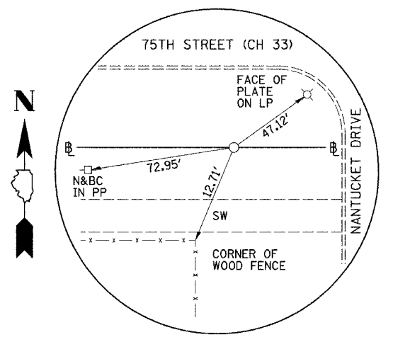
PI STA. 525+59.20 75TH STREET (CH 33) (5/8" I-ROD)
