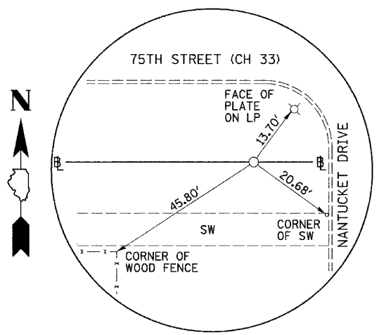
PI STA. 525+92.32 75TH STREET (CH 33) (5/8" I-ROD)
