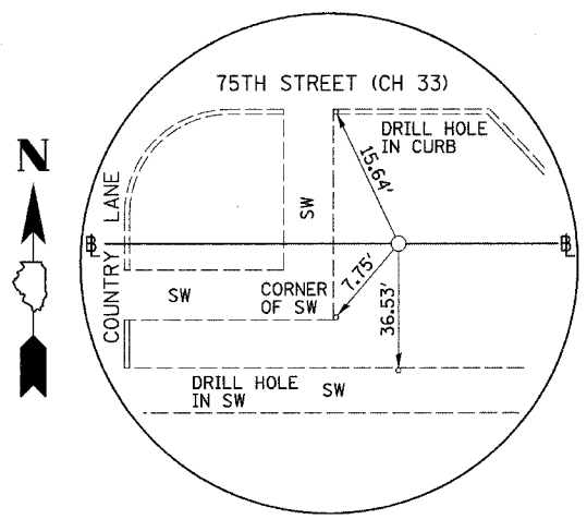
PI STA. 519+52.69 75TH STREET (CH 33) (5/8" I-ROD)
