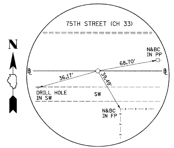
PI STA. 520+11.09 75 TH STREET (CH 33) (5/8" I-ROD)
