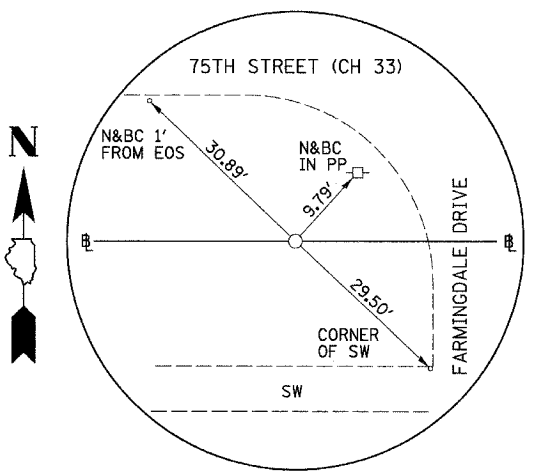
PI STA. 532+89.33 75TH STREET (CH 33) (5/8" I-ROD)
