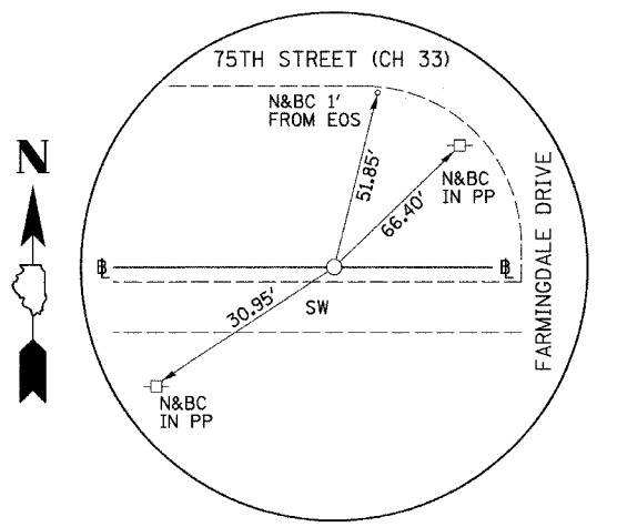
PI STA. 532+33.41 75TH STREET (CH 33) (5/8" I-ROD)
