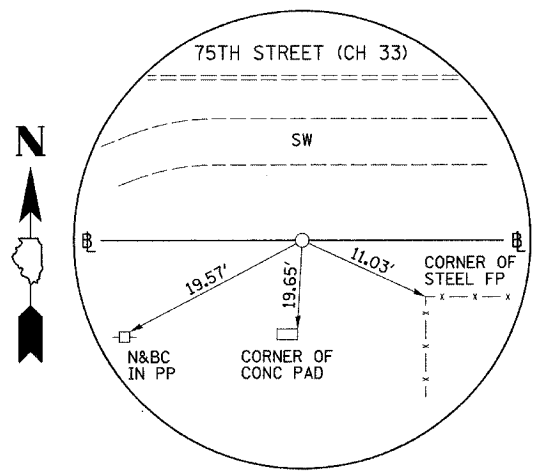
PI STA. 527+01.89 75TH STREET (CH 33) (5/8" I-ROD)
