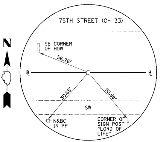
PI STA. 538+89.49 75TH STREET (CH 33) (5/8" I-ROD)
