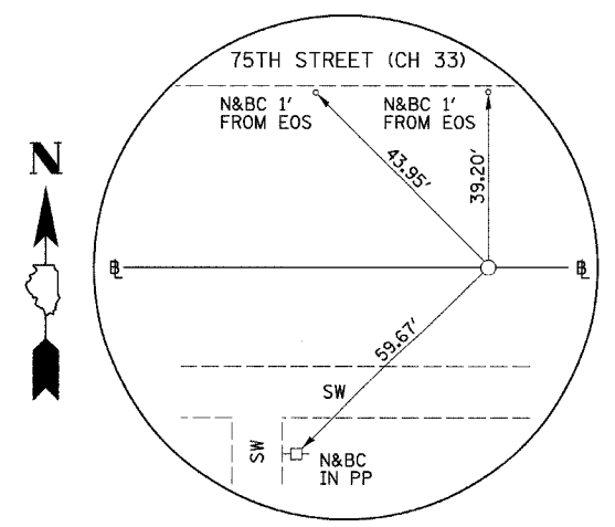
PI STA. 534+40.03 75TH STREET (CH 33) (5/8" I-ROD)
