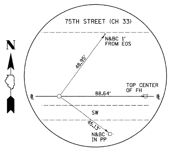
PI STA. 536+77.13 75TH STREET (CH 33) (5/8" I-ROD)
