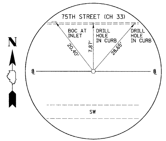
PI STA. 528+02.67 75TH STREET (CH 33) (5/8" I-ROD)
