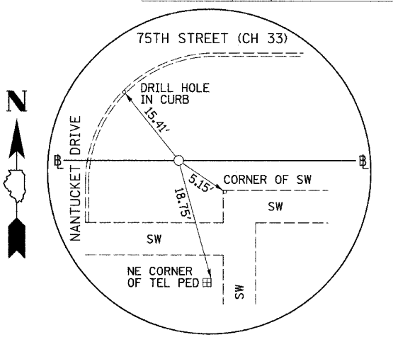
PI STA. 526+54.53 75TH STREET (CH 33) (5/8" I-ROD)
