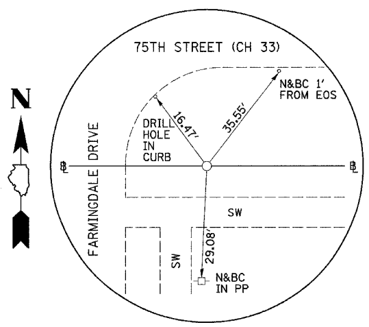
PI STA. 533+87.06 75TH STREET (CH 33) (5/8" I-ROD)
