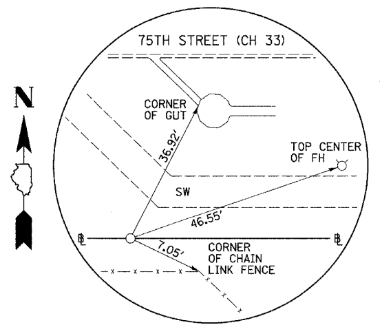
PI STA. 528+94.12 75TH STREET (CH 33) (5/8" I-ROD)
