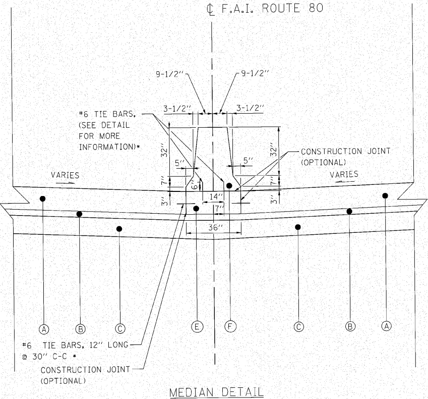
MEDIAN DETAIL F.A.I. ROUTE 80 CONCRETE BARRIER, DOUBLE FACE, 42" HEIGHT
