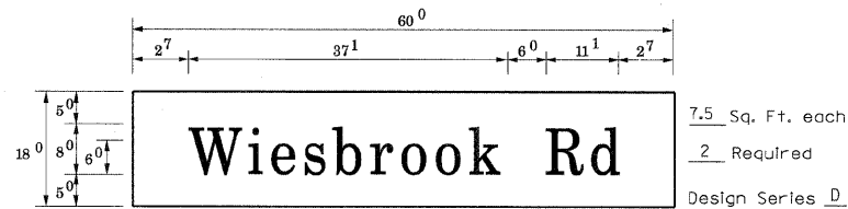
PANEL SIGN DESIGN TYPE 1
