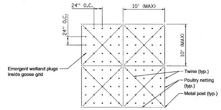
PLAN 1" = 8'
