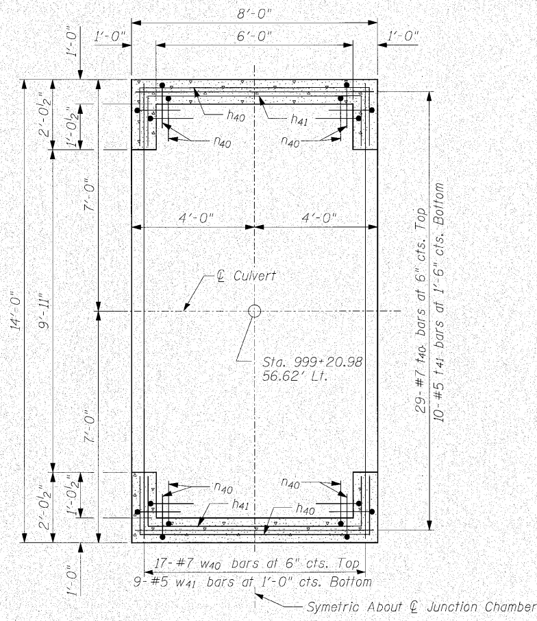
BOTTOM SLAB PLAN
