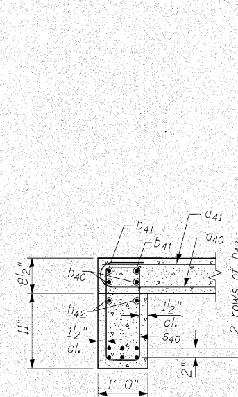
DETAIL B
