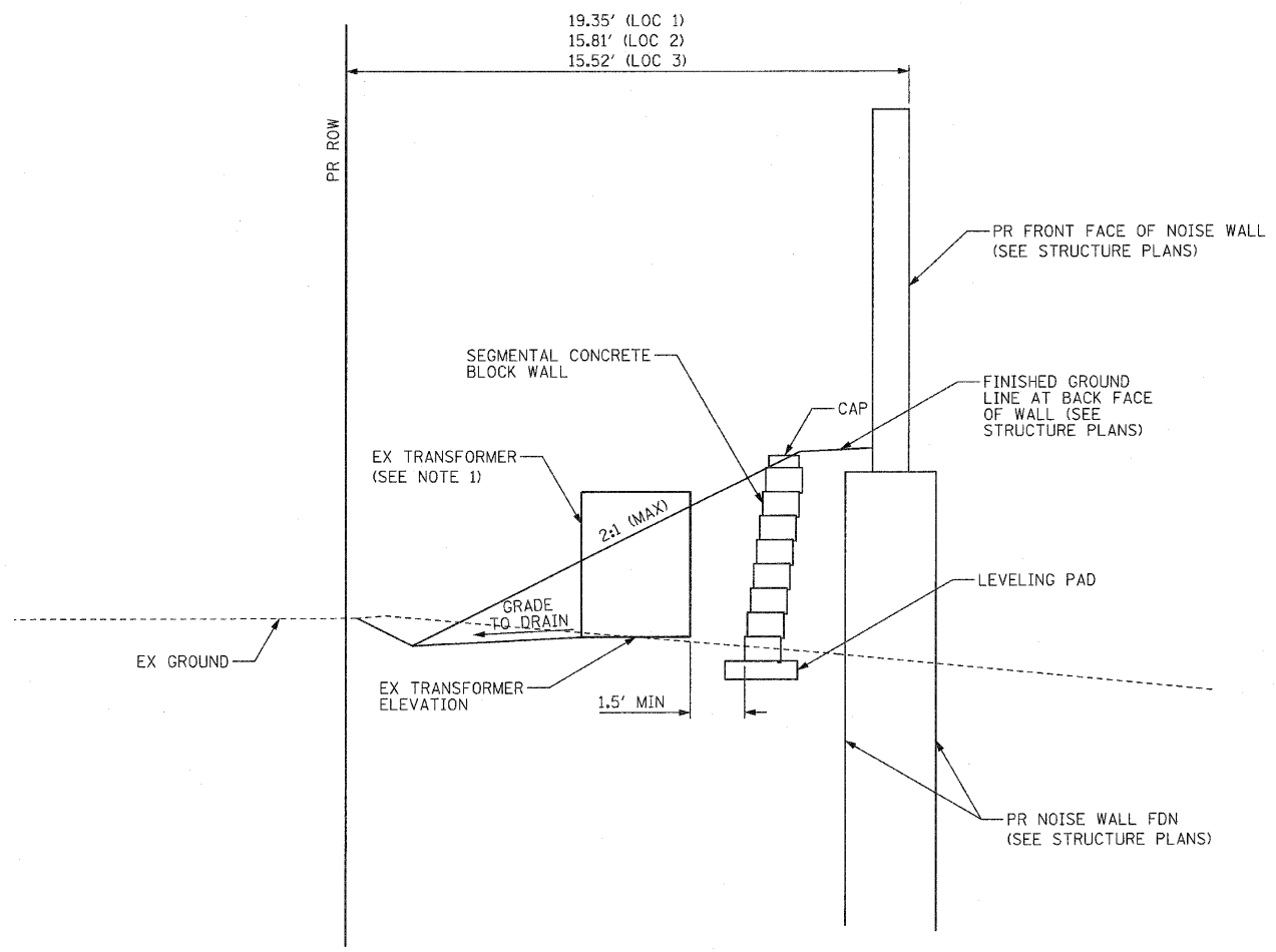
TYPICAL SECTION
