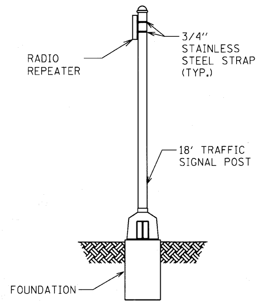
RADIO REPEATER INSTALLATION DETAILS
