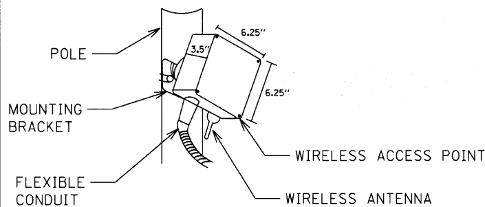
WIRELESS ACCESS POINT INSTALLATION DETAILS
