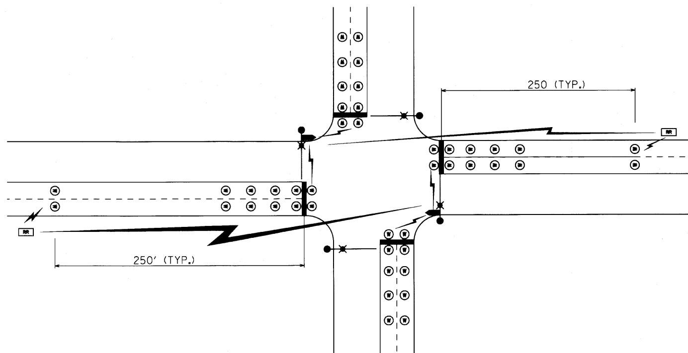
TYPICAL LAYOUT FOR ADVANCED WIRELESS DETECTION
