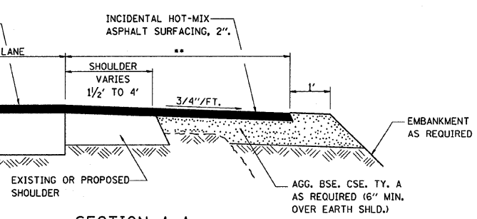
SECTION A-A MAILBOX TURNOUT DETAILS
