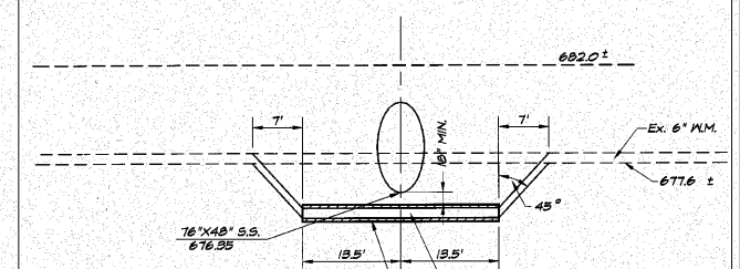
ADJUSTING WATER MAIN, 6" STA. 10+49.0 S.S. OUTFALL
