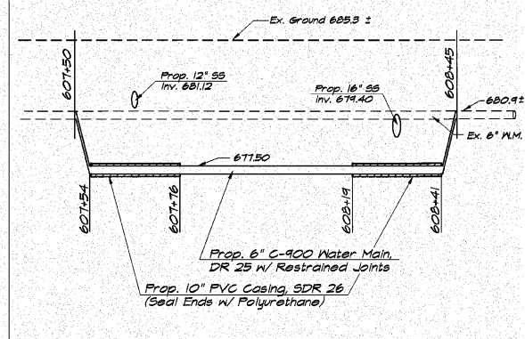
ADJUSTING WATER MAIN, 6" CLAY AND BELLE STREETS
