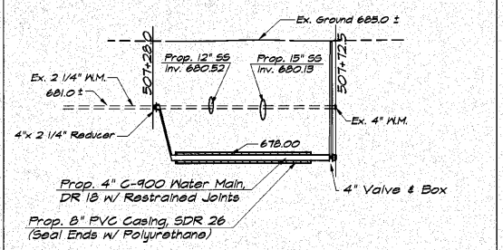
ADJUSTING WATER MAIN, 4" BELLE AND WEST STREETS
