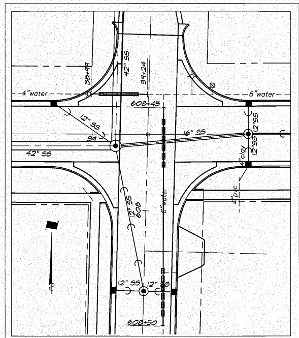
ADJUSTING WATER MAIN, 6" CLAY AND BELLE STREETS
