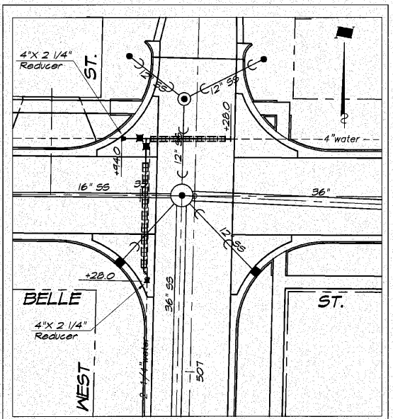
ADJUSTING WATER MAIN, 4" BELLE AND WEST STREETS
