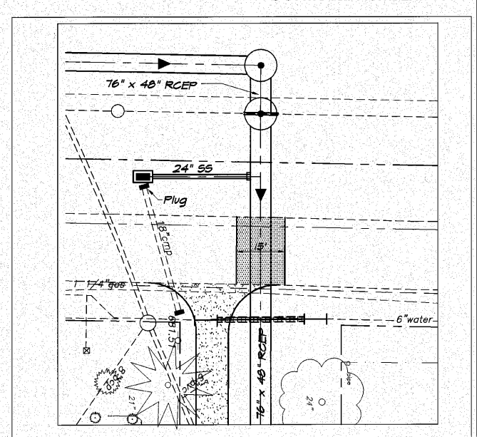
ADJUSTING WATER MAIN, 6" STA. 10+49.0 S.S. OUTFALL
