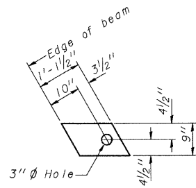
FABRIC BEARING PAD FIXED (Exterior)
