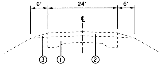
EXISTING TYPICAL SECTION - IL ROUTE 150 MS 0.0 TO 18.28
