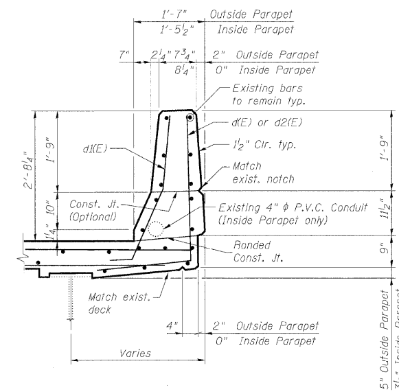
PROPOSED PARAPET SECTION
