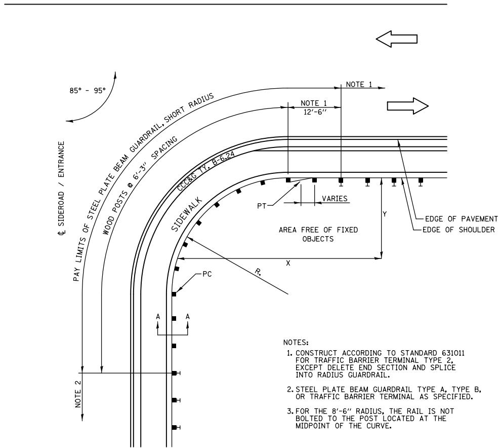
PLAN VIEW SHORT RADIUS GUARDRAIL DETAIL NOT TO SCALE
