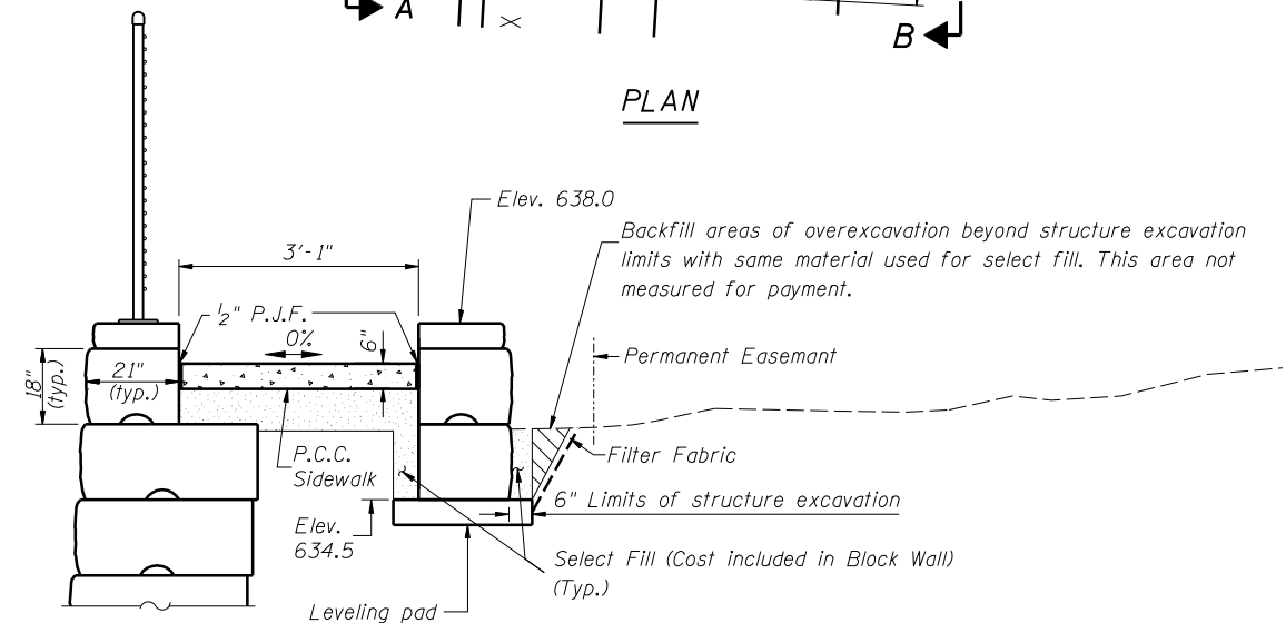
SECTION C-C
