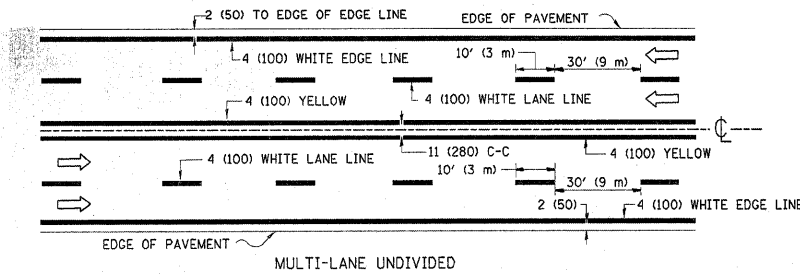
MULTI-LANE UNDIVIDED
