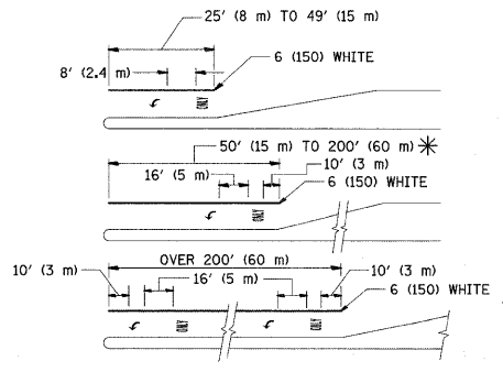
FULL SIZE LETTERS 8' (2.4 m) AND ARROWS SHALL BE USED. * AREA = 15.6 SQ. FT. (1.5 m 2 ) ONLY AREA = 20.8 SQ. FT. (1.9 m 2 ) * TURN LANES IN EXCESS OF 400' (120 m) IN LENGTH MAY HAVE AN ADDITIONAL SET OF ARROW - "ONLY" INSTALLED MIDWAY BETWEEN THE OTHER TWO SETS OF ARROW - "ONLY". TYPICAL LEFT (OR RIGHT) TURN LANE
