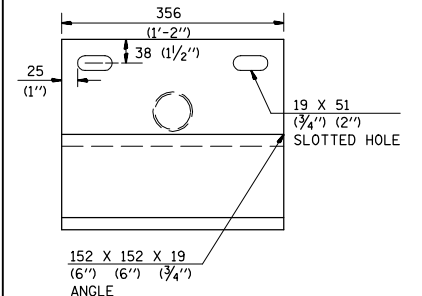
PLAN VIEW OF SUPPORT (IF SPECIFIED)
