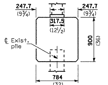
BRIDGE PIER MOUNT
