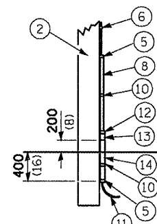
POLE, WOOD
