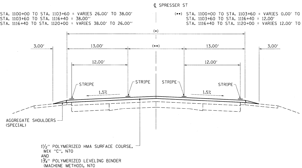
PROPOSED TYPICAL SECTION STA. 1100+00 TO STA. 1120+00
