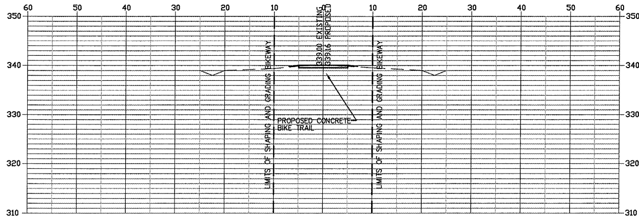
STATION 1004+00
