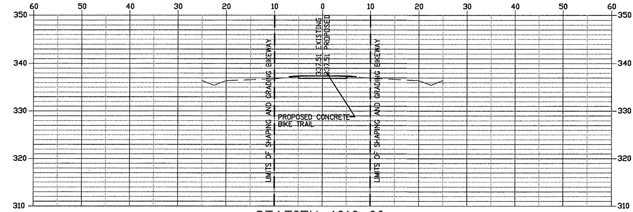
STATION 1010+00
