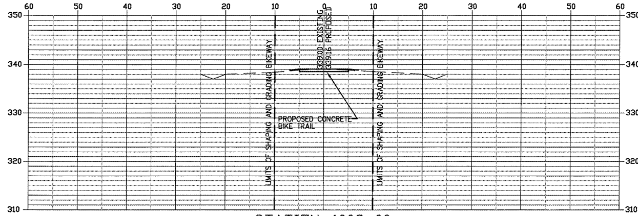
STATION 1002+00
