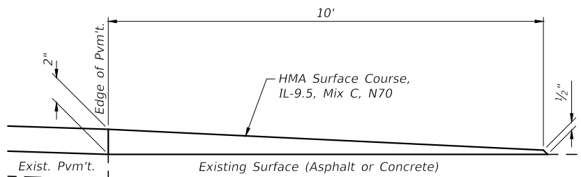
SECTION A-A PRIVATE ENTRANCE - ASPHALT (Est. No. = 0)
