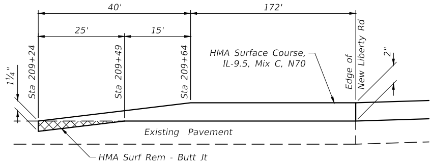
PROFILE - BAY CITY ROAD - STA. 125+15 LT.
