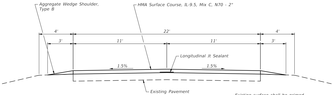
TYPICAL SECTION
