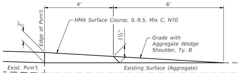
SECTION A-A PRIVATE ENTRANCE - AGGREGATE (Est. No. = 20)
