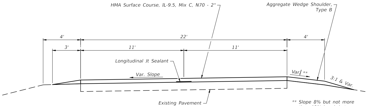
TYPICAL SECTION THRU CURVE
