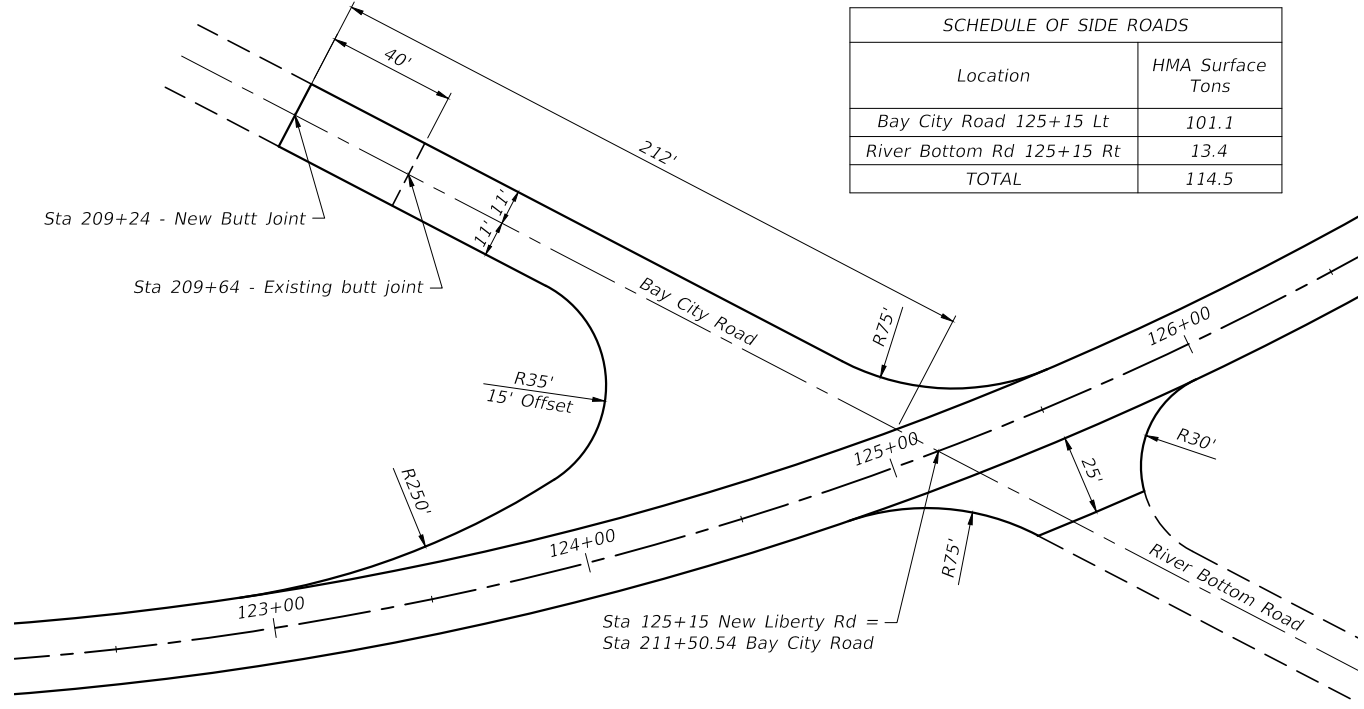
SIDE ROAD DETAILS
