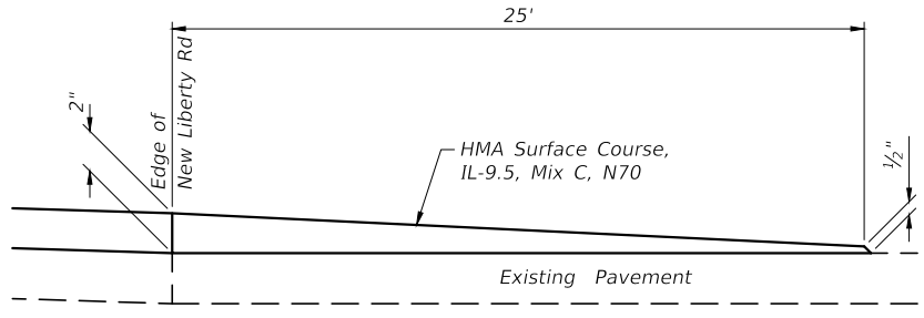
PROFILE - RIVER BOTTOM ROAD - STA. 125+15 RT.
