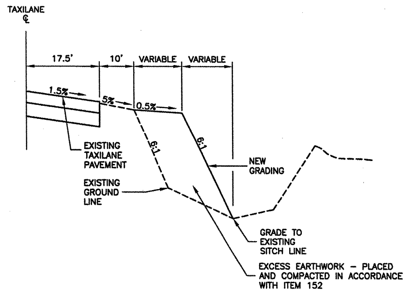
EXCESS EARTHWORK DISPOSAL AREA
