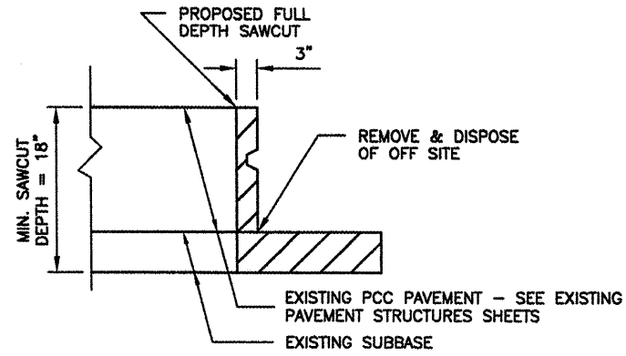
PCC PAVEMENT EDGE SAWING DETAIL
