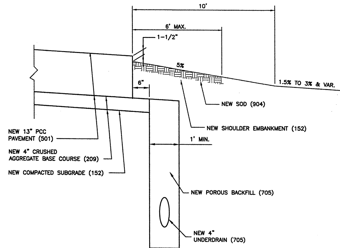
NEW TURF SHOULDER - TYPICAL SECTION
