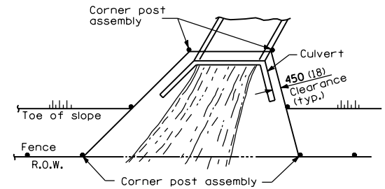
PLAN AT HEADWALL
