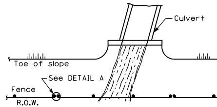
PLAN AT STREAM CROSSING
