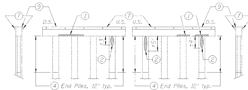
SOUTH ELEVATION EAST ELEVATION WEST ELEVATION NORTH ELEVATION PILE BENT 5
