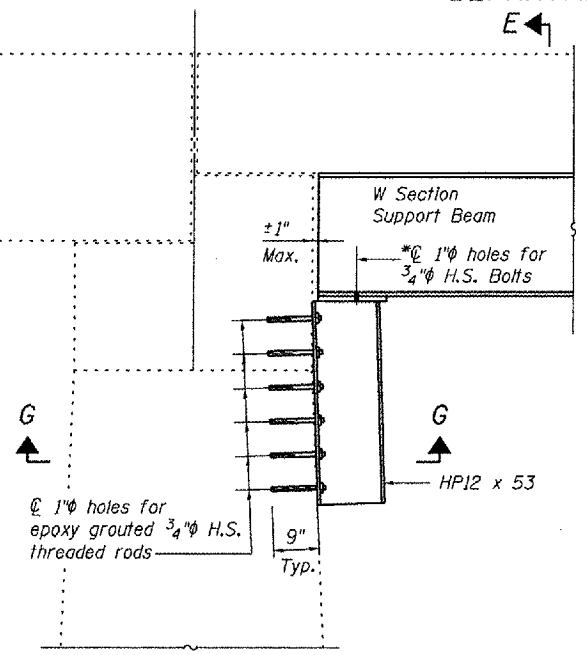
SECTION B-B (At Pier 7)
