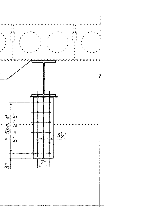
SECTION E-E
