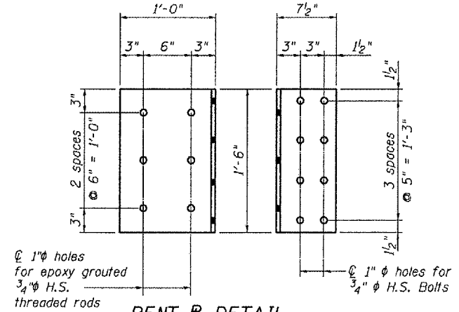
BENT PLATE DETAIL
