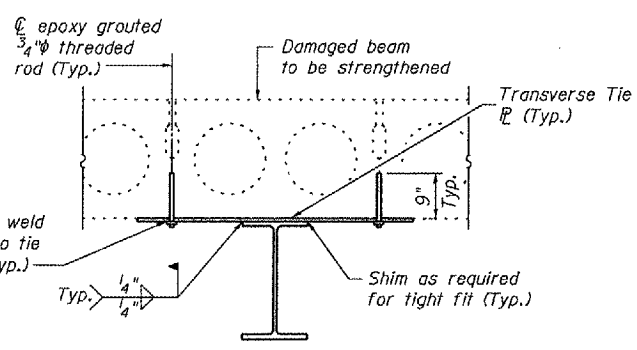
SECTION I-I
