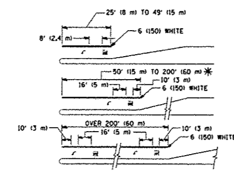
TYPICAL PAINTED MEDIAN MARKING TYPICAL LEFT (OR RIGHT) TURN LANE
