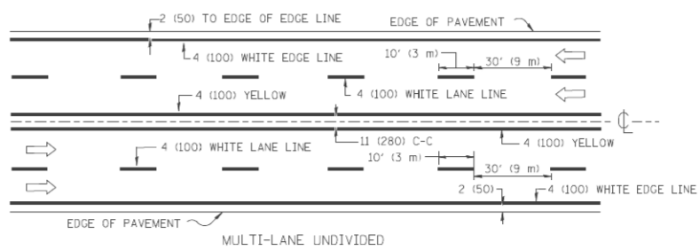
MULTI-LANE UNDIVIDED
