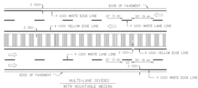
MULTI-LANE DIVIDED WITH MOUNTABLE MEDIAN
