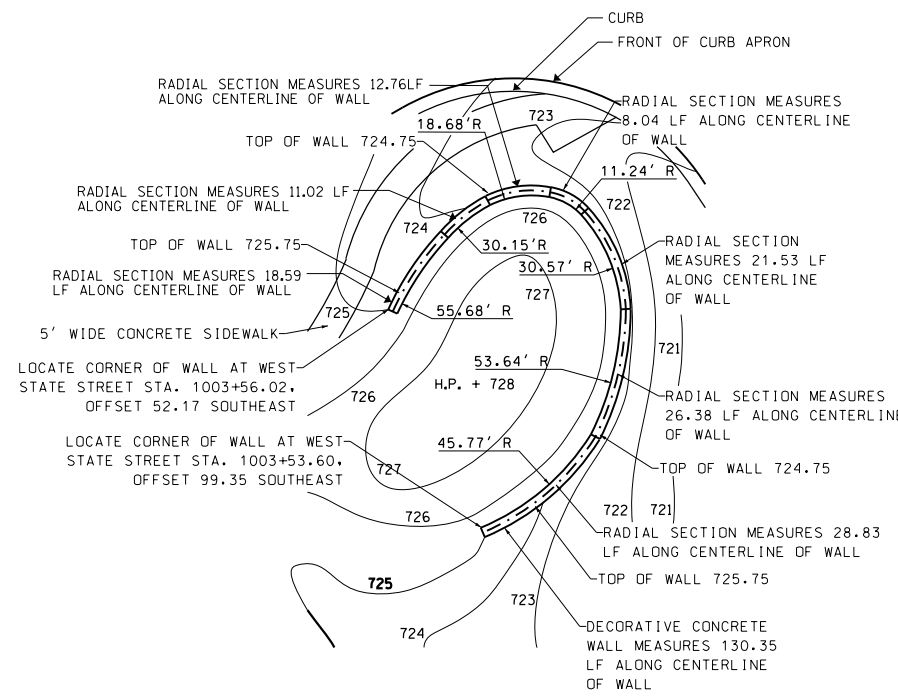
5 DECORATIVE CONCRETE BLOCK SEAT WALL AT NORTH TRIANGLE DETAIL L-6 NTS
