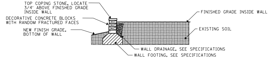
3 DECORATIVE CONCRETE BLOCK WALL DETAIL 2 L-6 NTS
