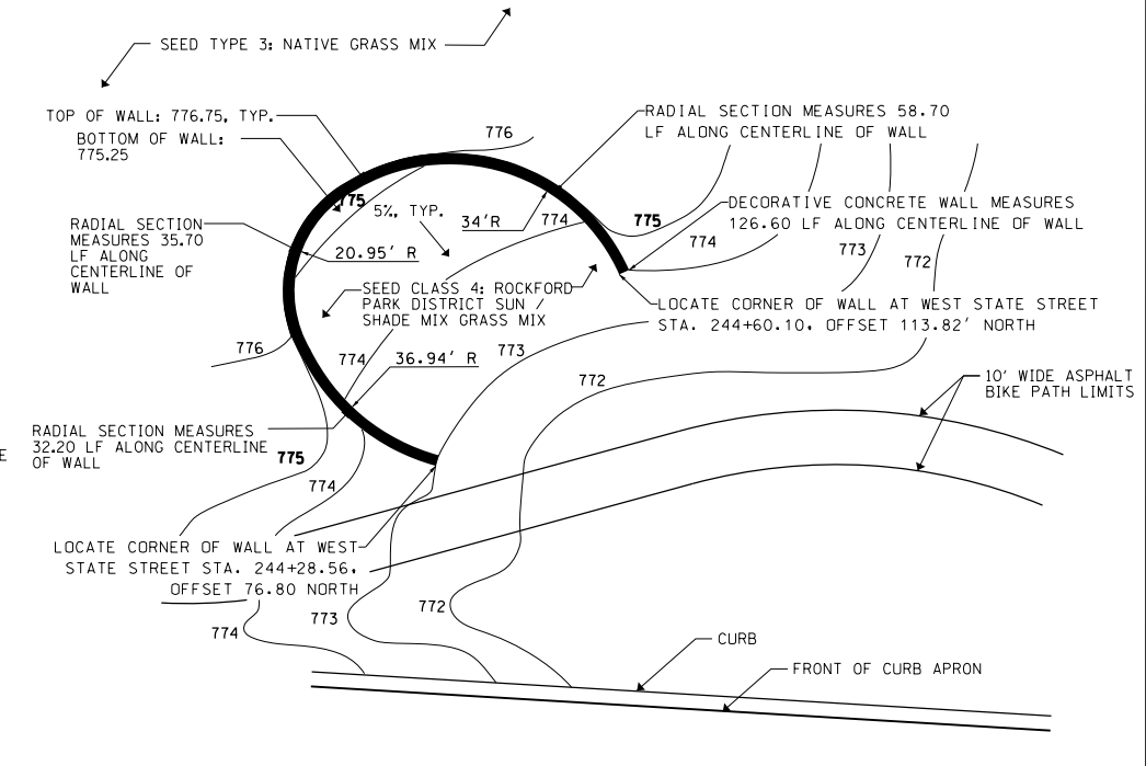
6 DECORATIVE CONCRETE BLOCK SEAT WALL AT NORTH INDEPENDENCE DETAIL L-6 NTS
