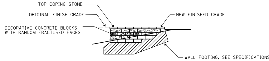
2 DECORATIVE CONCRETE BLOCK WALL DETAIL 1 L-6 NTS
