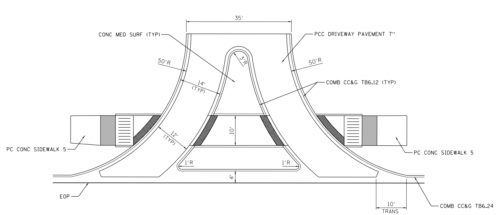
DRIVEWAY DETAIL STA 354+96.71 RT
