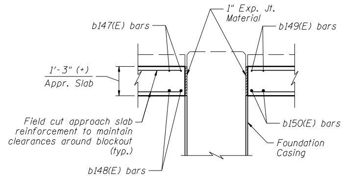
SECTION X-X
