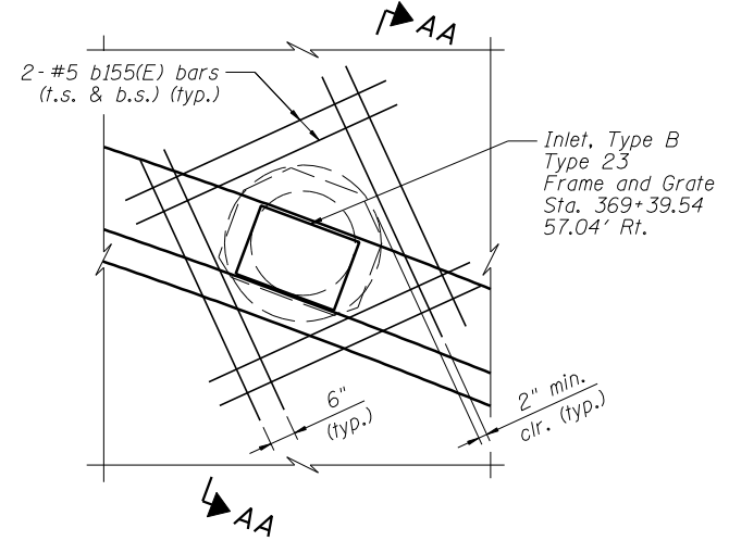
DETAIL 3B
