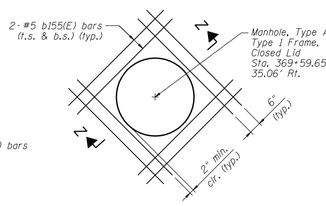
DETAIL 2B
