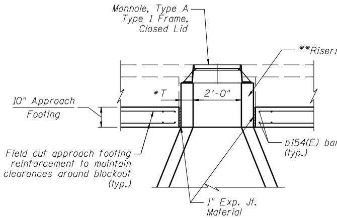
SECTION Y-Y
