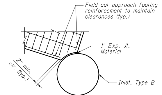
DETAIL 3A
