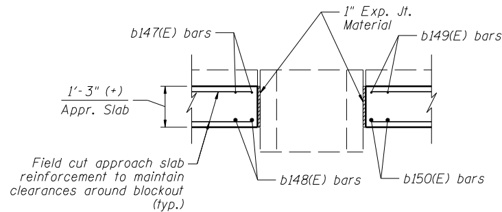
SECTION W-W
