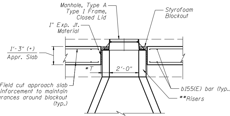
SECTION Z-Z
