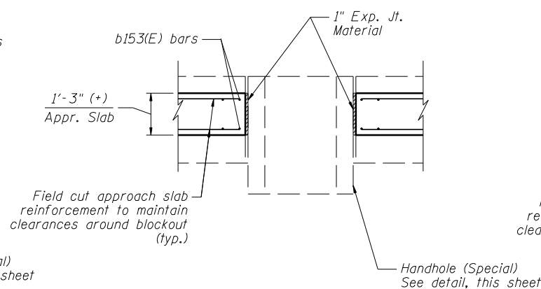
SECTION CC-CC
