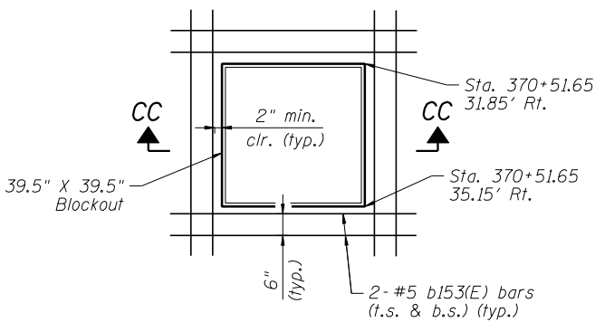
DETAIL 4B
