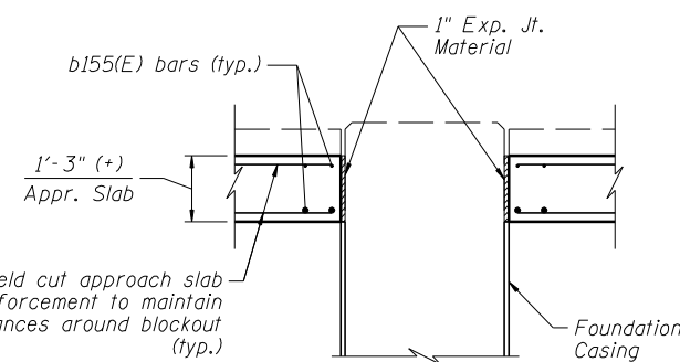
SECTION DD-DD
