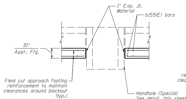
SECTION BB-BB
