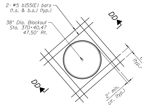
DETAIL 5A
