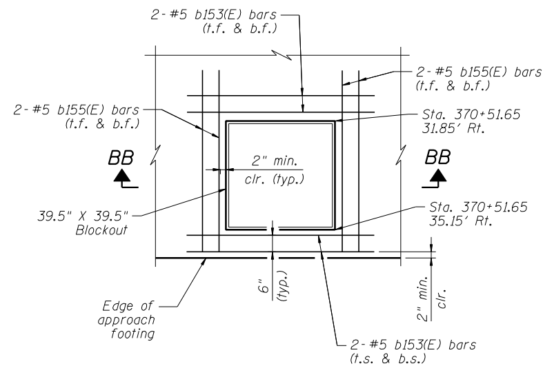
DETAIL 4A
