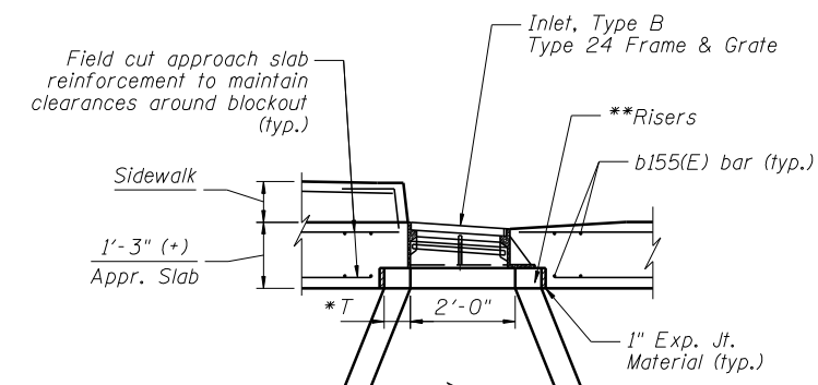
SECTION EE-EE
