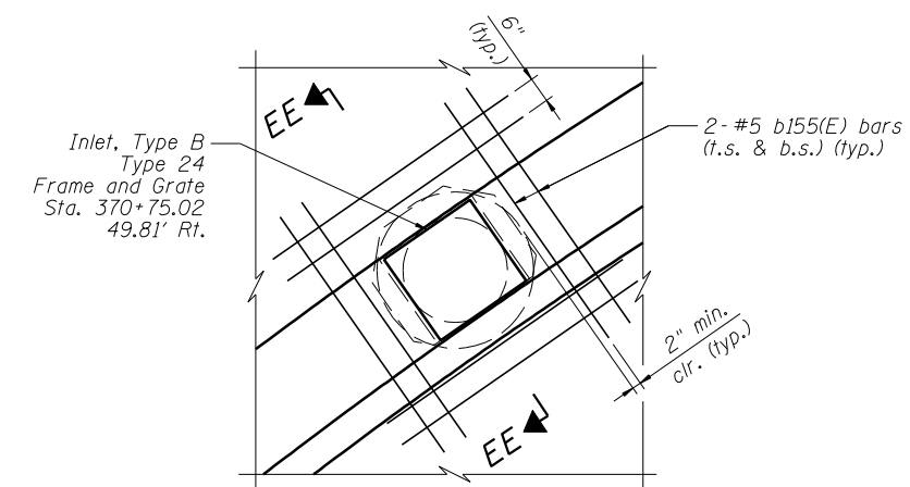
DETAIL 6
