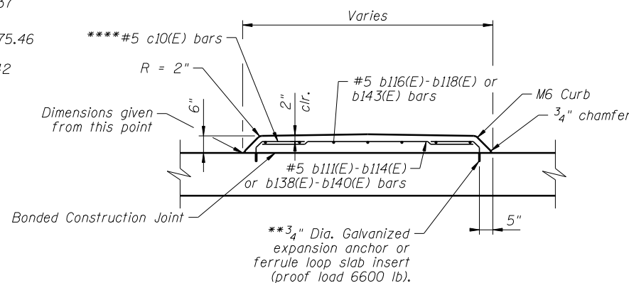
SECTION H-H
