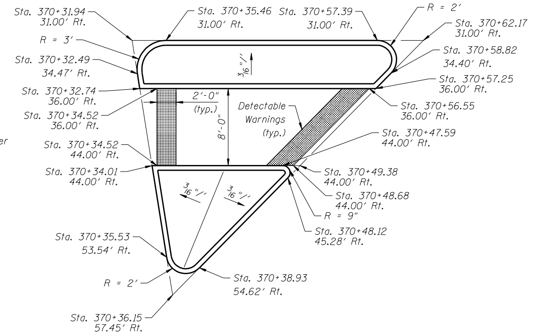
NORTH TRAFFIC ISLAND LAYOUT
