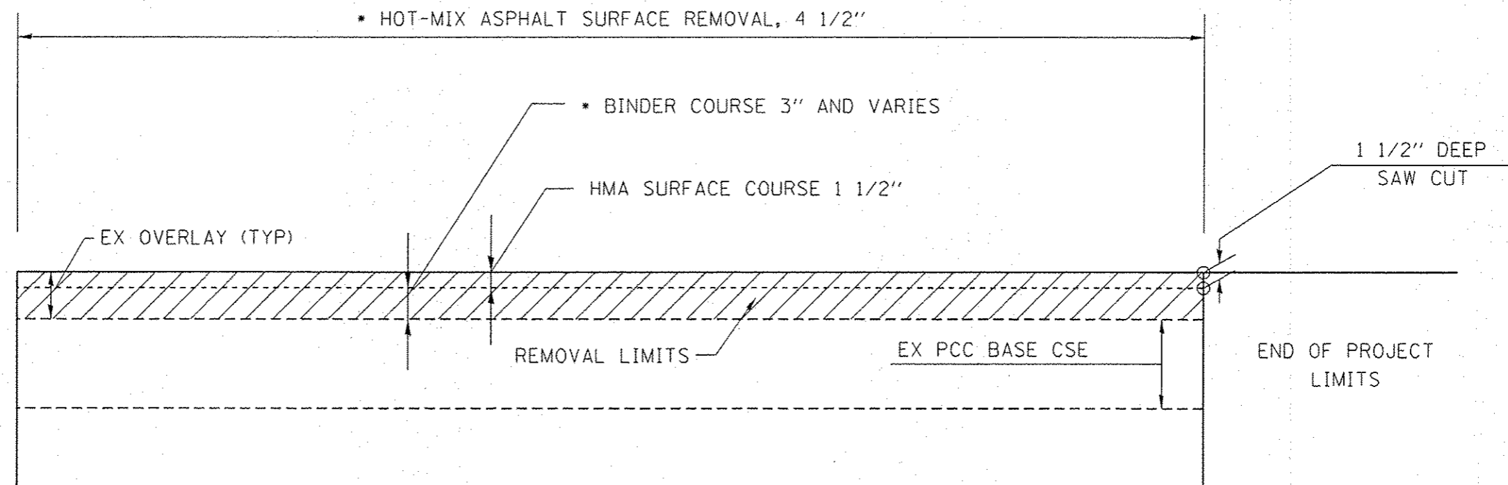
BUTT JOINT DETAIL
