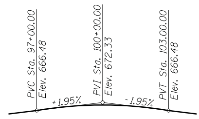
PROFILE GRADE
