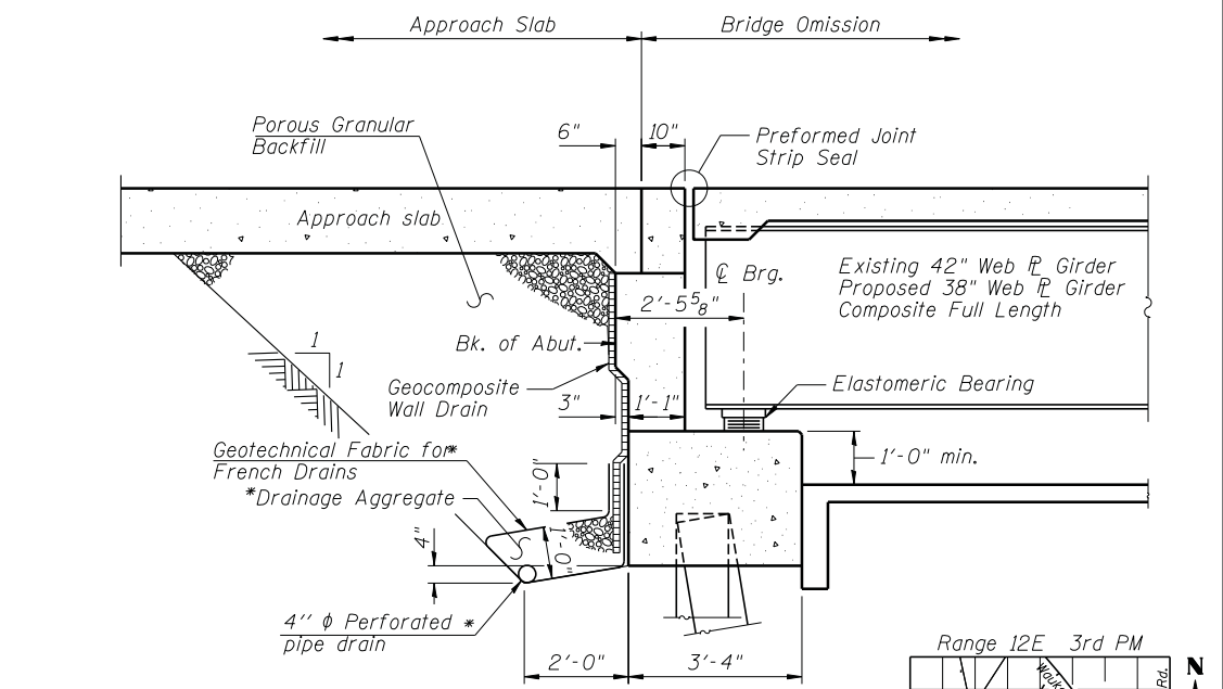
SECTION THRU ABUTMENTS (Horiz. dim. @ Rt. L's)
